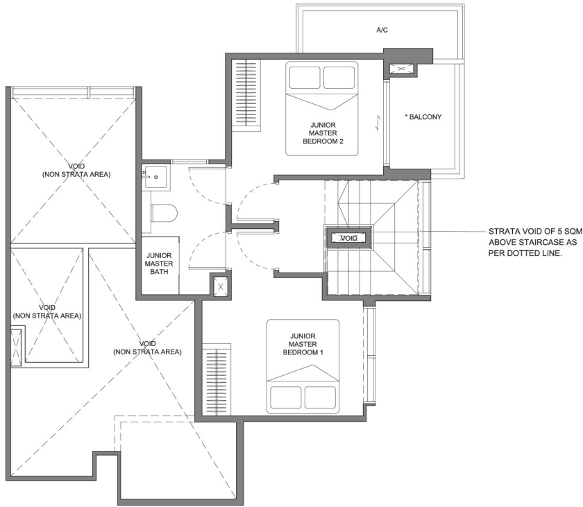
UPPER LEVEL
